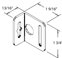
Hold Down Bracket (available upon request) Item # 80-37053-xx 03-Black, 09-Vanilla, 11-White, 38-Bronze
