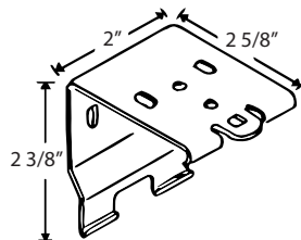
Installation Bracket Large Cassette Item # 100-37000-82
