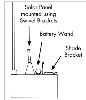
Figure B Shade with Solar Panel Mounted using Supplied Swivel Brackets
