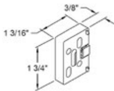
Spacer Block 50-03-142 The Spacer Block used behind an extension bracket is item 50-03-143
