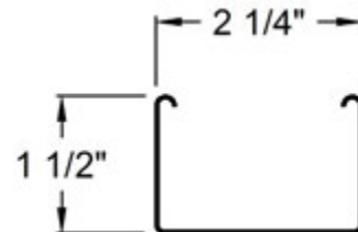
Low Profile Headrail
